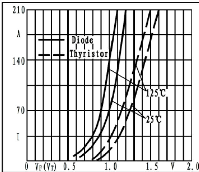
Fig2. Forward characteristics
